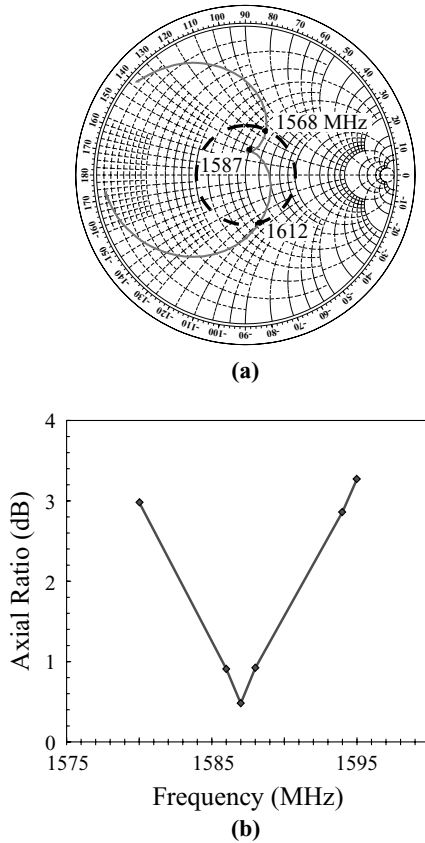
FIGURE 5.64 Measured (a) input impedance and (b) axial ratio of the antenna shown in Figure 5.63; \epsilon_r = 4.4 , h = 1.6 mm, D = 32 mm, \ell = 30 mm, \ell_s = 8.5 mm, \ell_t = 27 mm, w_t = 0.8 mm, and w_f = 3.0 mm. (From Ref. 19, © 1998 IEEE, reprinted with permission.)
