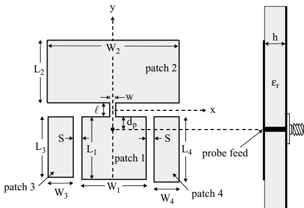
FIGURE 7.1 Geometry of a proposed broadband microstrip antenna with directly coupled and parasitic patches. (From Ref. 3, © 1999 John Wiley & Sons, Inc.)
