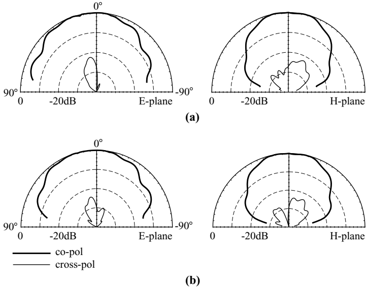
FIGURE 7.59 Measured E -plane ( x - z plane) and H -plane ( y - z plane) radiation patterns for the antenna shown in Figure 7.57 with \alpha = 30^\circ . (a) f = 1725 MHz, (b) f = 1763 MHz. (From Ref. 28, © 1999 John Wiley & Sons, Inc.)
