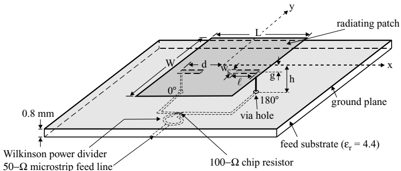
FIGURE 7.64 Geometry of a broadband dual capacitively fed microstrip antenna with reduced cross-polarization radiation. (From Ref. 10, © 2000 John Wiley & Sons, Inc.)
