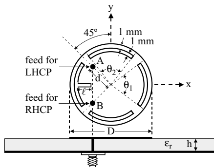
FIGURE 9.22 Geometry of a single-feed, slotted circular microstrip antenna for dual-band CP operation. (From Ref. 10, © 1998 IEE, reprinted with permission.)
