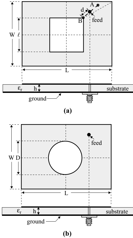
FIGURE 4.65 Geometries of a compact dual-frequency rectangular microstrip antenna with (a) a square slot and (b) a circular slot.
