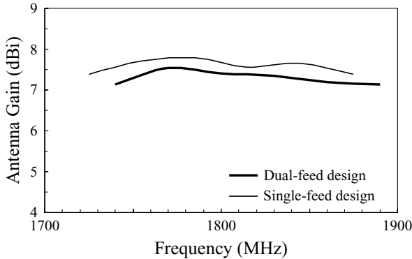
FIGURE 7.70 Measured on-axis antenna gain for the antenna studied in Figure 7.68. (From Ref. 10, © 2000 John Wiley & Sons, Inc.)
