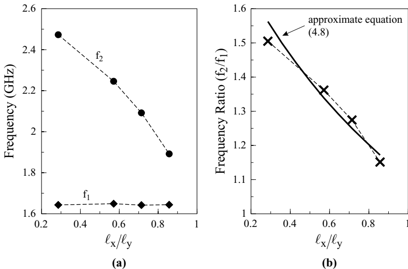
FIGURE 4.68 (a) The first two resonant frequencies f_1 and f_2 and (b) frequency ratio f_2/f_1 against the slit ratio l_x/l_y ; \epsilon_r = 4.4 , h = 1.6 mm, R = 16 mm, and l_y = 14 mm ( = 0.875R ). (From Ref. 34, © 1998 John Wiley & Sons, Inc.)
