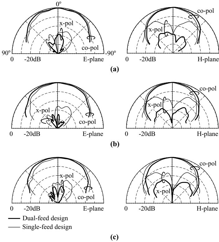
FIGURE 7.66 Measured E -plane ( x - z plane) and H -plane ( y - z plane) radiation patterns for the antenna studied in Figure 7.65. (a) f = 1530 MHz, (b) f = 1600 MHz, (c) f = 1655 MHz. (From Ref. 10, © 2000 John Wiley & Sons, Inc.)
