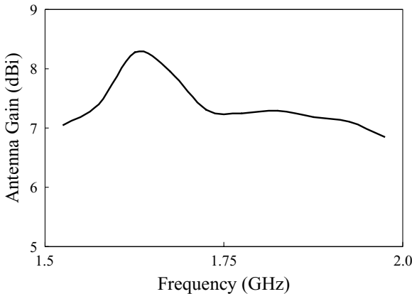
FIGURE 7.22 Measured antenna gain in the broadside direction of the antenna studied in Figure 7.20. (From Ref. 17, © 2000 John Wiley & Sons, Inc.)
