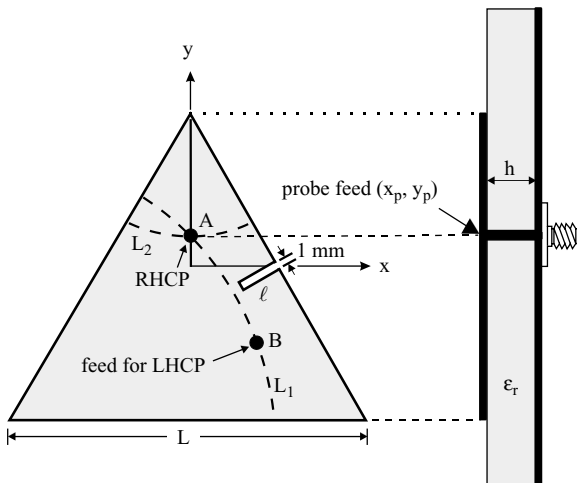
FIGURE 5.19 Geometry of a single-feed triangular microstrip antenna with a single slit for CP radiation. (From Ref. 6, © 1998 IEE, reprinted with permission.)
