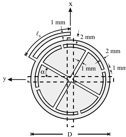
FIGURE 5.70 Geometry of a circular microstrip patch with a modified cross slot and a bent tuning stub for compact CP operation. (From Ref. 22, © 1998 IEE, reprinted with permission.)
