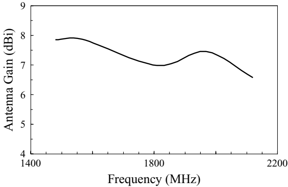
FIGURE 7.25 Measured antenna gain in the broadside direction of the antenna studied in Figure 7.24. (From Ref. 18, © 2000 John Wiley & Sons, Inc.)
