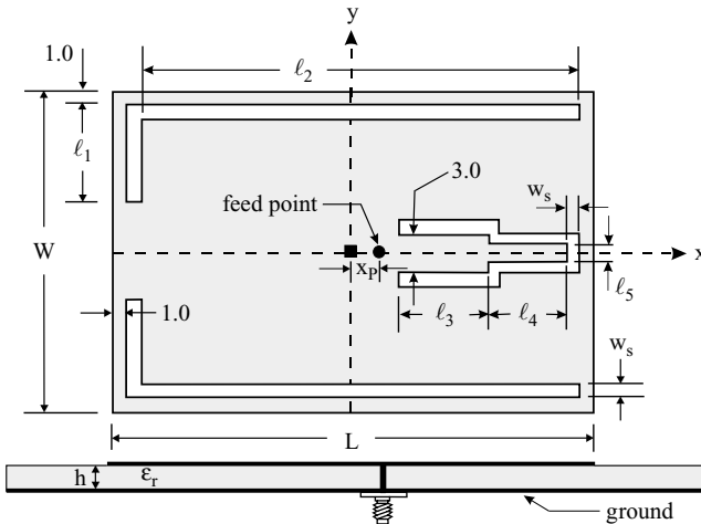
FIGURE 7.39 Geometry of a broadband rectangular microstrip antenna with a pair of right-angle slots and a modified U-shaped slot. The dimensions given in the figure are in millimeters. (From Ref. 23, © 2000 IEEE, reprinted with permission.)
