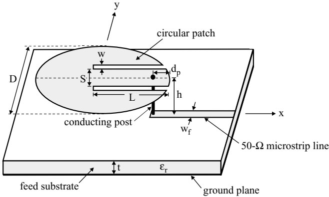
FIGURE 7.19 Geometry of a broadband probe-fed circular-E microstrip antenna. (From Ref. 17, © 2000 John Wiley & Sons, Inc.)
