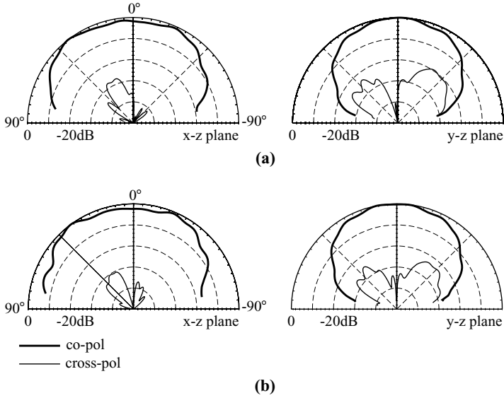
FIGURE 7.41 Measured x - z plane ( E -plane) and y - z plane ( H -plane) radiation patterns for antenna 1 studied in Figure 7.40. (a) f = 1844 MHz, (b) f = 1900 MHz. (From Ref. 23, © 2000 IEEE, reprinted with permission.)
