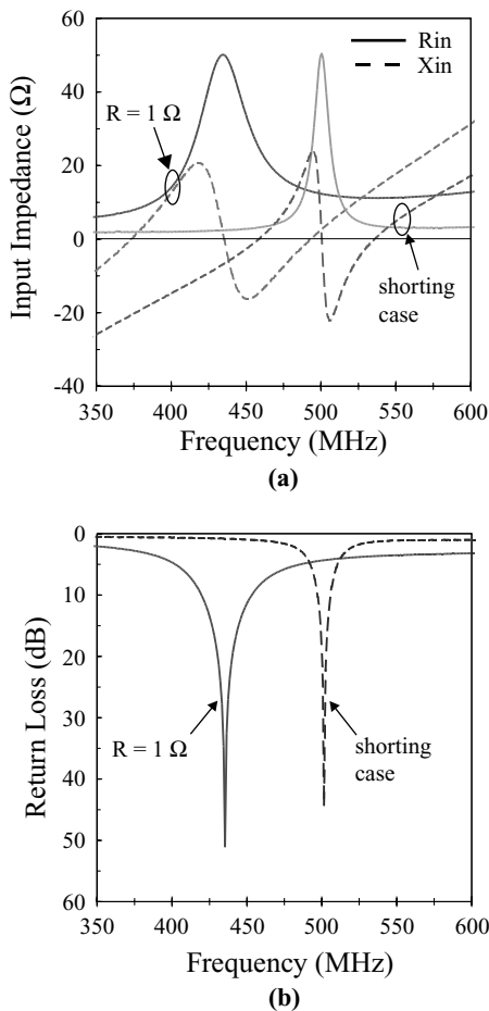
FIGURE 3.39 Measured (a) input impedance and (b) return loss for a triangular microstrip antenna with a shorting-pin loading or a chip-resistor loading. Antenna parameters are given in Table 3.7. (From Ref. 20, © 1997 John Wiley & Sons, Inc.)
