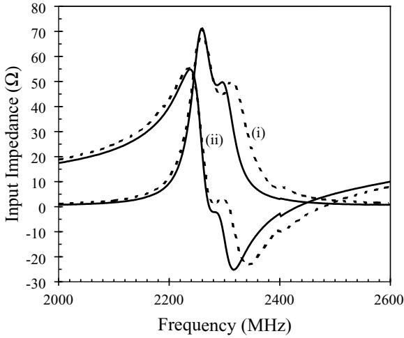
FIGURE 6.6 Measured input impedance for the antenna shown in Figure 6.5. Curve (i) is for an antenna with a high-permittivity superstrate and slits in the patch, and curve (ii) is for an antenna with a nearly square patch. Parameters and performance of antennas (i) and (ii) are given, respectively, by antennas 5 and 7 in Table 6.2. (From Ref. 2, © 1998 IEE, reprinted with permission.)
