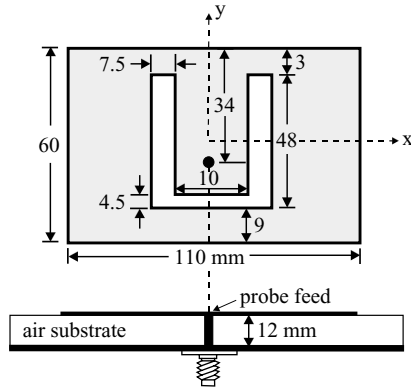
FIGURE 7.6 Geometry of a broadband probe-fed rectangular microstrip antenna with a U-shaped slot.
