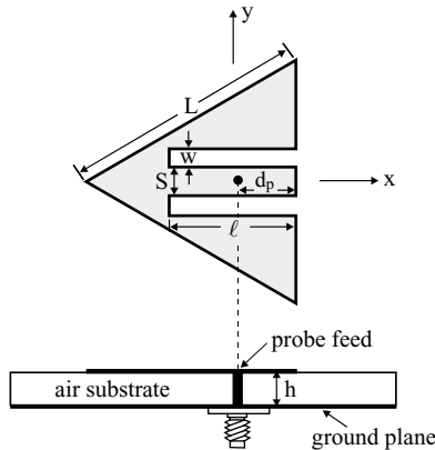
FIGURE 7.26 Geometry of a broadband probe-fed triangular-E microstrip antenna.
