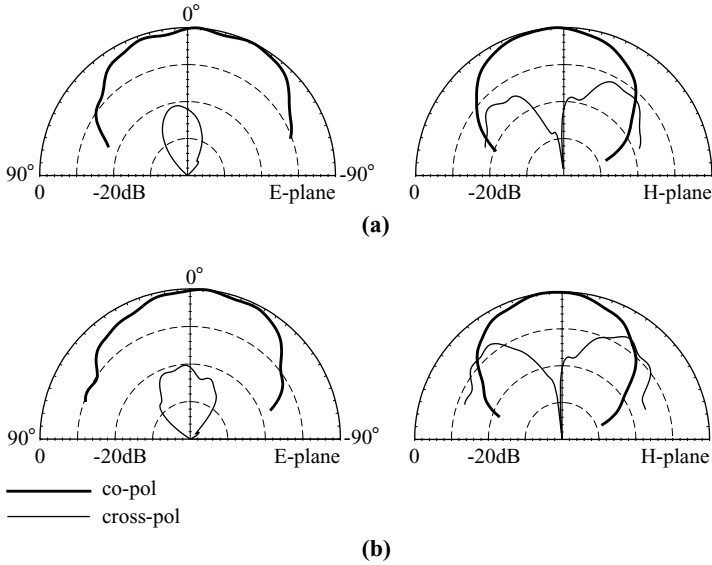
FIGURE 7.21 Measured E -plane ( x - z plane) and H -plane ( y - z plane) radiation patterns for the antenna studied in Figure 7.20. (a) f = 1575 MHz, (b) f = 1875 MHz. (From Ref. 17, © 2000 John Wiley & Sons, Inc.)
