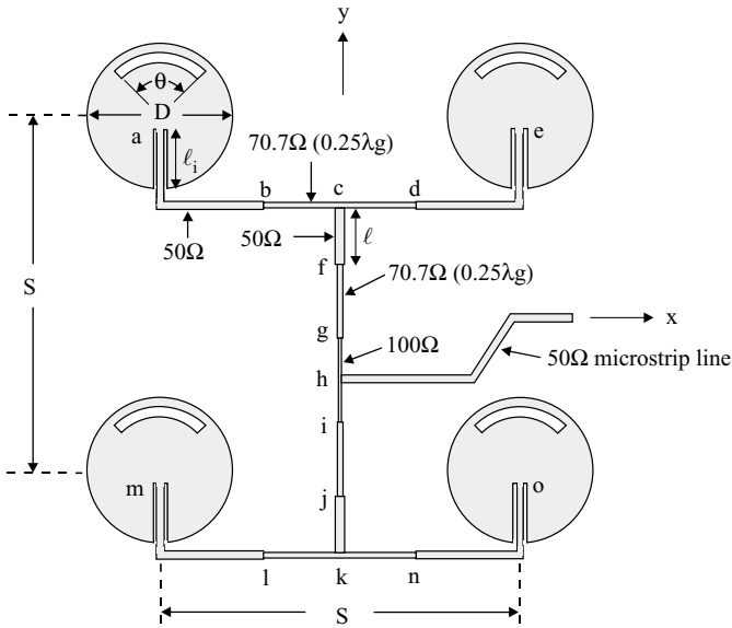
FIGURE 4.28 Geometry of a 2 \times 2 dual-frequency microstrip subarray with dual-frequency feed network and slotted circular patches. The slotted circular patches have the same geometry as given in Figure 4.13.
