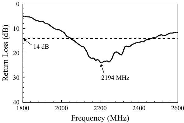
FIGURE 7.29 Measured return loss for the antenna shown in Figure 7.28; L = 60 mm, W = 90 mm, h_1 = 2 mm, h_2 = 21 mm, and ground-plane size = 180 \times 120 mm 2 .
