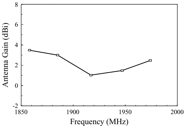
FIGURE 7.52 Measured antenna gain in the broadside direction for the antenna studied in Figure 7.50. (From Ref. 26, © 1998 IEE, reprinted with permission.)
