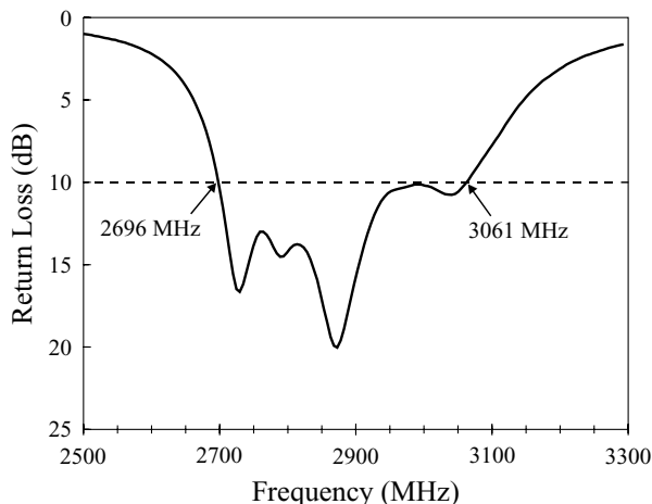
FIGURE 7.2 Measured return loss against frequency for the antenna shown in Figure 7.1; \epsilon_r = 4.4 , h = 1.6 mm, L_1 = 26.6 mm, L_2 = 24.4 mm, L_3 = 26.47 mm, L_4 = 27 mm, W_1 = 16 mm, W_2 = 40 mm, W_3 = W_4 = 10 mm, S = 2 mm, \ell = 2 mm, w = 0.2 mm, and d_p = 1.2 mm. (From Ref. 3, © 1999 John Wiley & Sons, Inc.)
