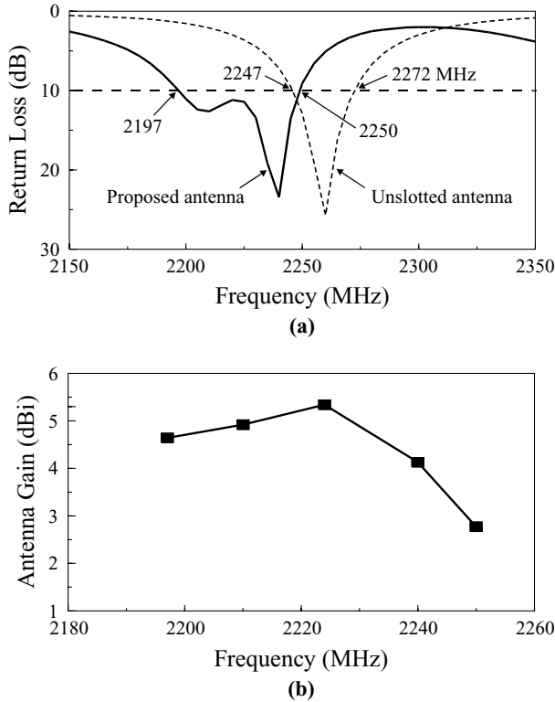
FIGURE 7.43 (a) Measured return loss and (b) peak antenna gain against frequency for the antenna shown in Figure 7.39 with a Rogers RO3003™ substrate; \epsilon_r = 3.0 , h = 1.524 mm, \ell_3 = 11 mm, \ell_4 = 7 mm, \ell_5 = 8 mm, w_s = 0.5 mm, and x_p = -9.4 mm. Other parameters are the same as for antenna 2 in Table 7.1. (From Ref. 23, © 2000 IEEE, reprinted with permission.)
