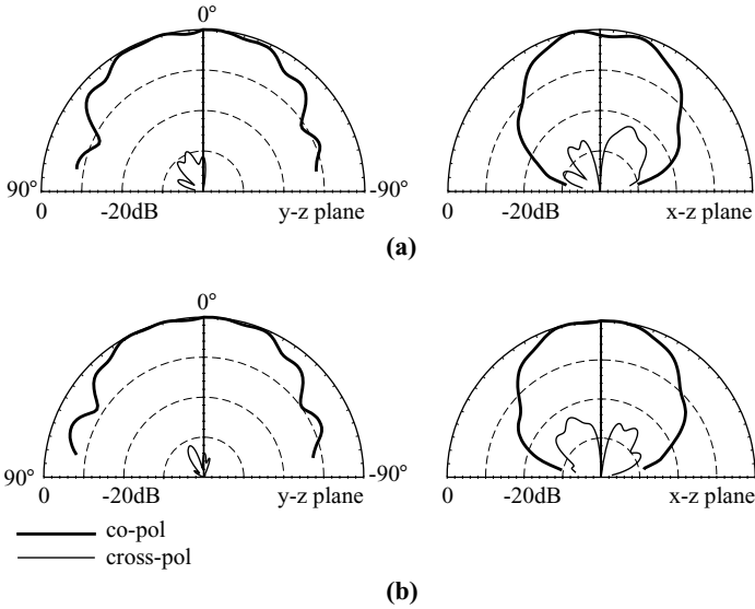
FIGURE 7.46 Measured y - z plane ( E -plane) and x - z plane ( H -plane) radiation patterns for the antenna studied in Figure 7.45. (a) f = 2148 MHz, (b) f = 2200 MHz. (From Ref. 24, © 1999 John Wiley & Sons, Inc.)
