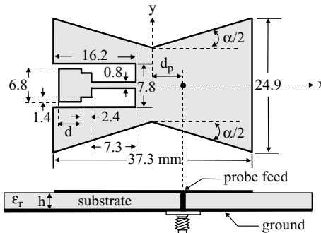
FIGURE 7.57 Geometry of a broadband bow-tie microstrip antenna with integrated reactive loading. The patch dimensions are in millimeters and not to scale; \epsilon_r = 4.4 , h = 1.6 \text{ mm} , and ground-plane size = 77 \times 55 \text{ mm}^2 . (From Ref. 28, © 1999 John Wiley & Sons, Inc.)
