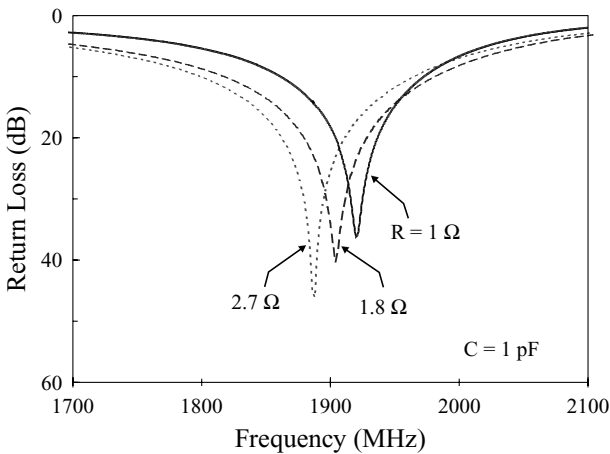
FIGURE 3.29 Variation of the measured return loss with the loading resistance; \epsilon_r = 4.4 , h = 1.6\ \text{mm} , d = 6.0\ \text{mm} , C = 1\ \text{pF} , (x_R, y_R) = (0, 5\ \text{mm}) , and (x_c, y_c) = (0, -5\ \text{mm}) .
