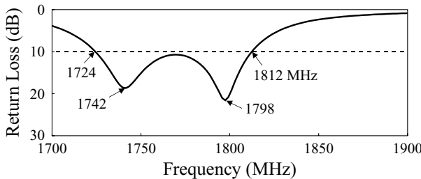
FIGURE 7.33 Measured return loss for the antenna shown in Figure 7.32; \epsilon_r = 4.4, h = 1.6 mm, l_3 = 9 mm, l_4 = 9 mm, l_5 = 7.5 mm, and ground-plane size = 60 \times 50 mm 2 ; other parameters are given in Figure 7.32. (From Ref. 21, © 1998 IEE, reprinted with permission.)
