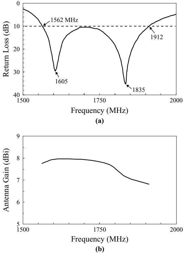
FIGURE 7.27 (a) Measured return loss and (b) antenna gain for the antenna shown in Figure 7.26; h = 16 mm, L = 79 mm, w = 6 mm, d_p = 15 mm, \ell = 41 mm, and ground-plane size = 150 \times 150 mm 2 .
