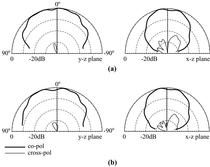
FIGURE 7.51 Measured y - z plane ( E -plane) and x - z plane ( H -plane) radiation patterns for the antenna studied in Figure 7.50. (a) f = 1885 MHz; (b) f = 1947 MHz. (From Ref. 26, © 1998 IEE, reprinted with permission.)
