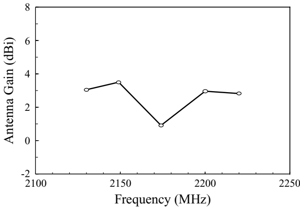
FIGURE 7.47 Measured antenna gain in the broadside direction for the antenna studied in Figure 7.45. (From Ref. 24, © 1999 John Wiley & Sons, Inc.)
