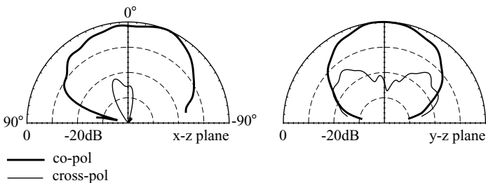
FIGURE 8.13 Measured radiation patterns at 1800 MHz for port 2 excitation (gap-coupled probe feed) of the antenna studied in Figure 8.10. (From Ref. 6, © 2000 John Wiley & Sons, Inc.)
