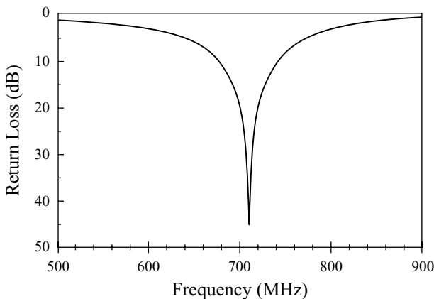
FIGURE 3.16 Measured return loss against frequency for the antenna studied in Figure 3.15 with d_p = 13.5 mm ( d_p/L = 0.36 ). (From Ref. 15, © 1997 IEE, reprinted with permission.)
