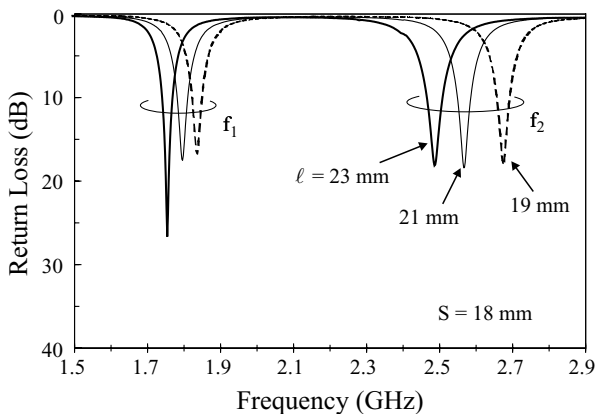
FIGURE 4.45 Measured return loss for various lengths of the embedded slots for the antenna shown in Figure 4.43; \epsilon_r = 4.4 , h = 1.6 mm, L = 50 mm, and ground-plane size = 75 \times 75 mm 2 . (From Ref. 23, © 1999 John Wiley & Sons, Inc.)
