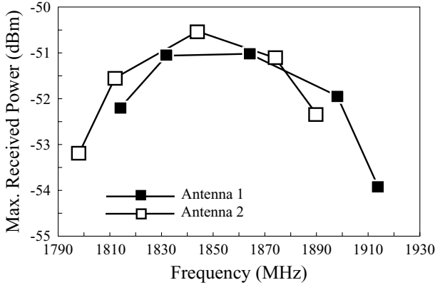
FIGURE 7.38 Measured maximum received power in the broadside direction for antennas 1 and 2 studied in Figure 7.37. (From Ref. 22, © 1999 John Wiley & Sons, Inc.)
