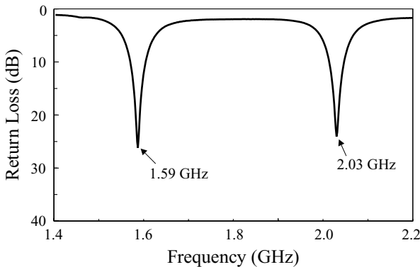
FIGURE 4.18 Measured return loss of the two-element dual-frequency microstrip array shown in Figure 4.17; \epsilon_r = 4.4 , h = 1.6 mm, D = 50 mm, l = 42 mm, S = 132.5 mm, and \theta = 100^\circ . (From Ref. 12, © 1999 IEE, reprinted with permission.)
