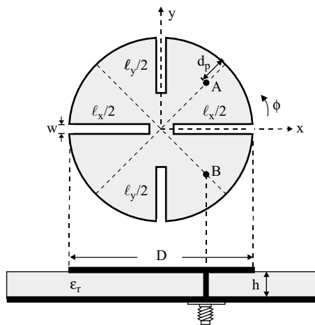
FIGURE 5.34 Geometry of a compact circular microstrip antenna with slits for CP radiation. (From Ref. 9, © 1998 John Wiley & Sons, Inc.)
