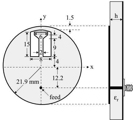
FIGURE 7.49 Geometry of a broadband circular microstrip antenna with an embedded reactive loading. The dimensions shown in the figure are not to scale. (From Ref. 26, © 1998 IEE, reprinted with permission.)
