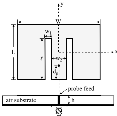
FIGURE 7.14 Geometry of a broadband E-shaped microstrip antenna. (From Ref. 15, © 2001 IEEE, reprinted with permission.)
