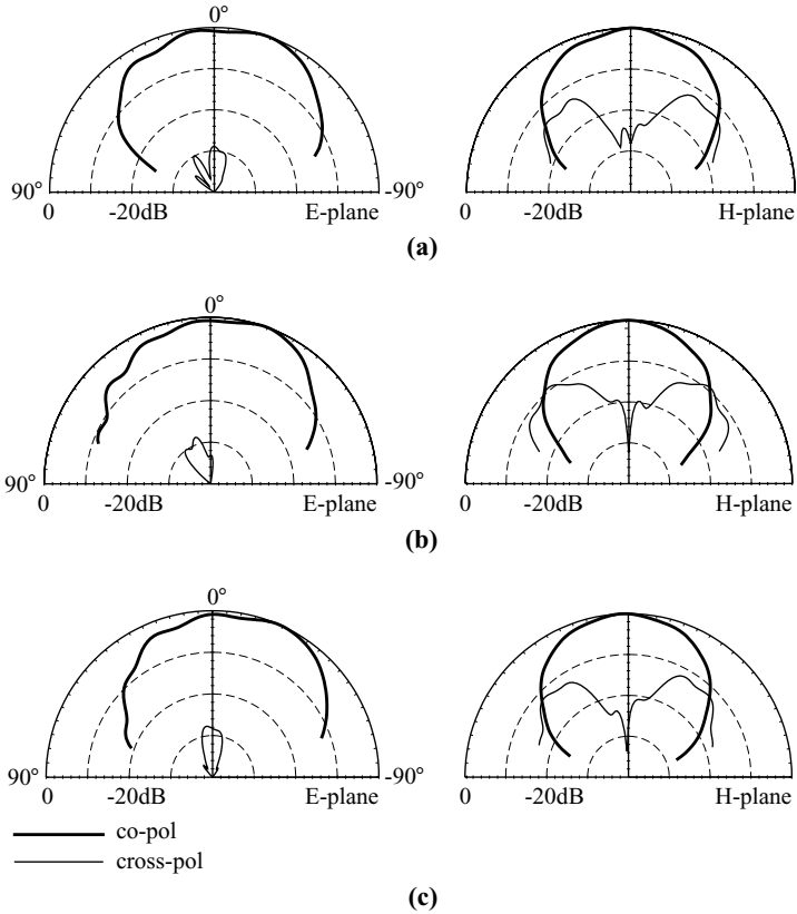
FIGURE 7.16 Measured E -plane ( y - z plane) and H -plane ( x - z plane) radiation patterns for antenna A studied in Figure 7.15. (a) f = 1485 MHz, (b) f = 1644 MHz, (c) f = 1740 MHz. (From Ref. 15, © 2001 IEEE, reprinted with permission.)
