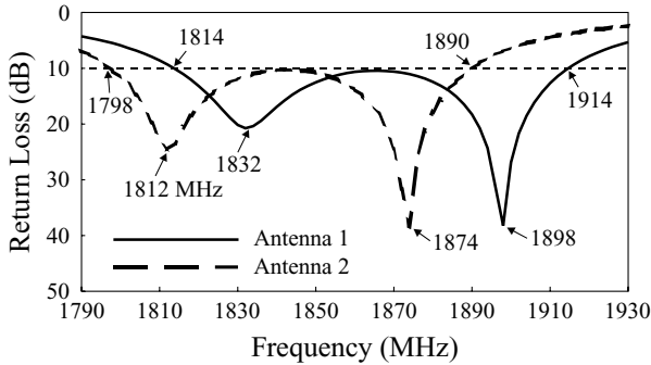
FIGURE 7.37 Measured return loss for the antenna shown in Figure 7.36; \epsilon_r = 4.4 , h = 1.6 mm, and ground-plane size = 60 \times 50 mm 2 . Antenna 1: \ell_t = 4.6 mm, x_p = 2.3 mm; antenna 2: \ell_t = 5.0 mm, x_p = -0.2 mm. Other parameters are given in Figure 7.36. (From Ref. 22, © 1999 John Wiley & Sons, Inc.)
