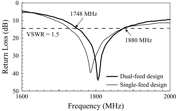
FIGURE 7.68 Measured return loss for the antenna shown in Figure 7.64; h = 17.2 mm, L = 48 mm, W = 72 mm, \ell = 14.8 mm, g = 3.2 mm, d = 19 mm, w_c = 1.0 mm, and ground-plane size = 150 \times 150 mm 2 . (From Ref. 10, © 2000 John Wiley & Sons, Inc.)
