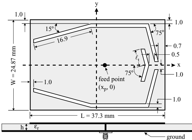
FIGURE 7.36 Geometry of a broadband slotted rectangular microstrip antenna. The dimensions given in the figure are in millimeters and not to scale. (From Ref. 22, © 1999 John Wiley & Sons, Inc.)
