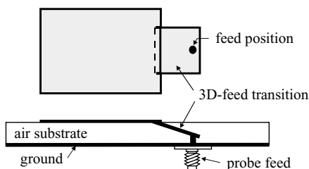
FIGURE 7.5 Geometry of a broadband microstrip antenna with a three-dimensional microstrip transition feed.
