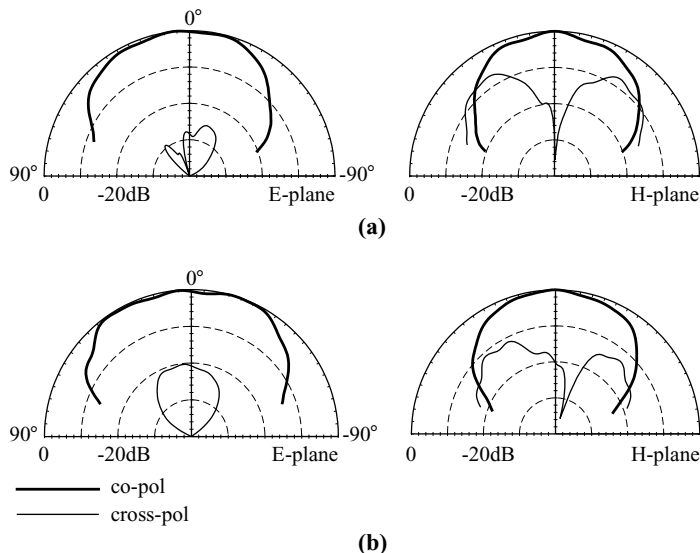
FIGURE 7.12 Measured E -plane ( y - z plane) and H -plane ( x - z plane) radiation patterns for the antenna studied in Figure 7.11. (a) f = 1563 MHz; (b) f = 1746 MHz. (From Ref. 14, © 1997 IEE, reprinted with permission.)
