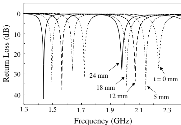
FIGURE 4.64 Measured return loss against frequency for the antenna shown in Figure 4.63; \epsilon_r = 4.4 , h = 1.6 mm, L = 37.7 mm, W = 28.4 mm, \ell = 12 mm.
