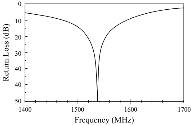
FIGURE 3.18 Measured return loss against frequency for the antenna shown in Figure 3.14(b); \epsilon_r = 3.0 , h = 0.762 mm, L = 21 mm, W = 14 mm, d_c = 1.65 mm, w_f = 1.9 mm, \ell = 16.9 mm, and g = 1 mm. (From Ref. 15, © 1997 IEE, reprinted with permission.)
