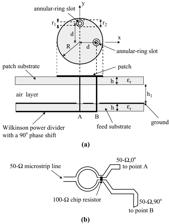
FIGURE 9.5 (a) Geometry of a single-layer, broadband circularly polarized microstrip antenna with two gap-coupled probe feeds; (b) the Wilkinson power divider with two outputs having a 90° phase shift for feeding the antenna. (From Ref. 6, © 2000 John Wiley & Sons, Inc.)
