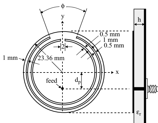
FIGURE 7.44 Geometry of a broadband circular microstrip antenna with two open-ring slots. The dimensions shown in the figure are not to scale. (From Ref. 24, © 1999 John Wiley & Sons, Inc.)
