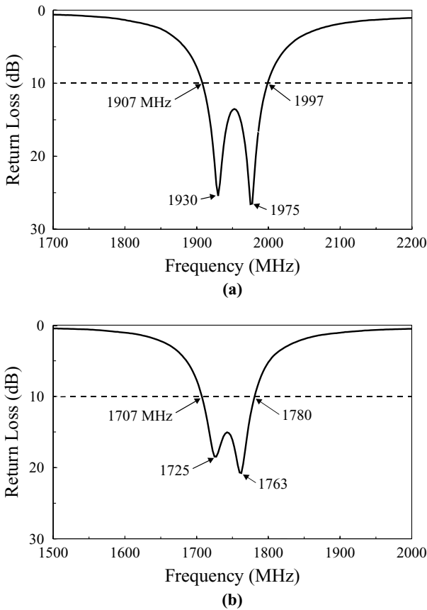
FIGURE 7.58 Measured return loss for the antenna shown in Figure 7.57. (a) \alpha = 0^\circ , (b) \alpha = 30^\circ . (From Ref. 28, © 1999 John Wiley & Sons, Inc.)
