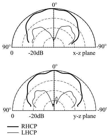
FIGURE 5.29 Measured radiation patterns of the antenna studied in Figure 5.27; f = 1526 MHz. (From Ref. 7, © 1999 IEEE, reprinted with permission.)
