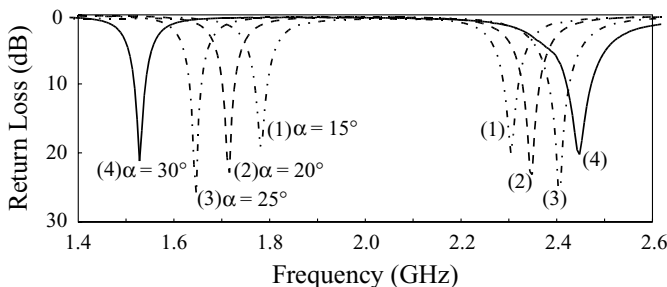
FIGURE 4.2 Measured return loss for the antenna shown in Figure 4.1; \epsilon_r = 4.4 , h = 1.6 mm, L = 37.3 mm, W = 24.87 mm, and \ell_s = 19 mm. (From Ref. 8, © 1998 IEE, reprinted with permission.)
