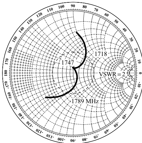
FIGURE 5.14 Measured input impedance for a square microstrip antenna with a slit [Figure 5.13(a)] for right-hand CP operation; \epsilon_r = 4.4 , h = 1.6 mm, L = 39.7 mm, l = 6 mm, and AC = 17 mm ( \cong 0.30AB ). (From Ref. 5, © 1998 John Wiley & Sons, Inc.)
