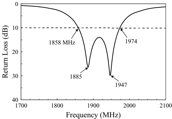
FIGURE 7.50 Measured return loss for the antenna shown in Figure 7.49; \epsilon_r = 4.4 , h = 1.6 mm, and ground-plane size = 75 \times 75 mm 2 . Patch dimensions are given in Figure 7.49. (From Ref. 26, © 1998 IEE, reprinted with permission.)
