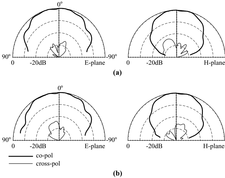
FIGURE 7.55 Measured E - and H -plane radiation patterns for the antenna studied in Figure 7.54 with \phi_c = 40^\circ . (a) f = 1885 MHz, (b) f = 1945 MHz. (From Ref. 27, © 1999 John Wiley & Sons, Inc.)
