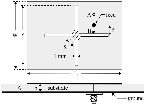
FIGURE 4.56 Geometry of a compact dual-frequency rectangular microstrip antenna with a pair of bent slots. (From Ref. 29, © 1998 IEE, reprinted with permission.)
