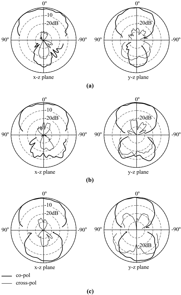
FIGURE 3.49 Measured radiation patterns for the antenna studied in Figure 3.48. (a) l = 0 , f = 2345 MHz; (b) l = 18 mm, f = 1980 MHz; (c) l = 20 mm, f = 1835 MHz. (From Ref. 23, © 2001 IEEE, reprinted with permission.)
