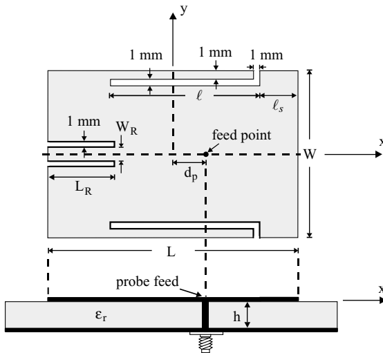
FIGURE 4.8 Geometry of a dual-frequency rectangular microstrip antenna with a pair of spur lines and an integrated reactive loading. (From Ref. 10, © 1999 John Wiley & Sons, Inc.)
