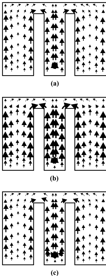
FIGURE 7.18 Simulated current distributions on the E-shaped patch of antenna A studied in Figure 7.15. (a) f = 1485 MHz, (b) f = 1644 MHz, (c) f = 1740 MHz. (From Ref. 15, © 2001 IEEE, reprinted with permission.)
