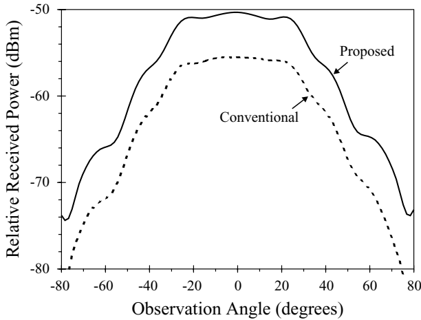
FIGURE 6.8 Measured radiation patterns in the \phi = 135^\circ plane at 2272 MHz for the proposed antenna (antenna 5 in Table 6.2) and for a conventional nearly square microstrip antenna (antenna 7 in Table 6.2). (From Ref. 2, © 1998 IEE, reprinted with permission.)
