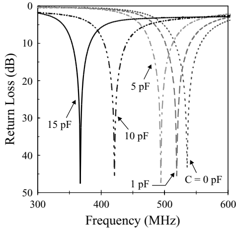
FIGURE 3.33 Measured return loss for the antenna shown in Figure 3.31 with a 1\text{-}\Omega chip resistor and a chip capacitor of various capacitances; antenna parameters are given in Table 3.5. (From Ref. 18, © 1998 John Wiley & Sons, Inc.)
