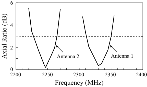
FIGURE 5.50 Measured axial ratio in the broadside direction for antennas 1 and 2 studied in Figure 5.49. (From Ref. 15, © 1998 IEE, reprinted with permission.)
