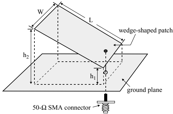
FIGURE 7.31 Geometry of a broadband probe-fed wedge-shaped microstrip antenna.
