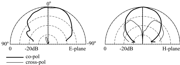
FIGURE 7.30 Measured radiation patterns at 2194 MHz for the antenna studied in Figure 7.29.
