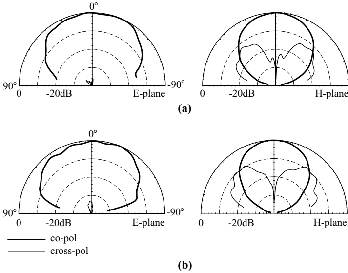
FIGURE 7.8 Measured radiation patterns for the antenna shown in Figure 7.6. (a) f = 1615 MHz; (b) f = 1955 MHz.
