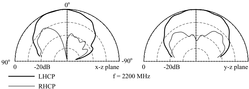
FIGURE 9.20 Measured radiation patterns at 2200 MHz for the antenna studied in Figure 9.17.
