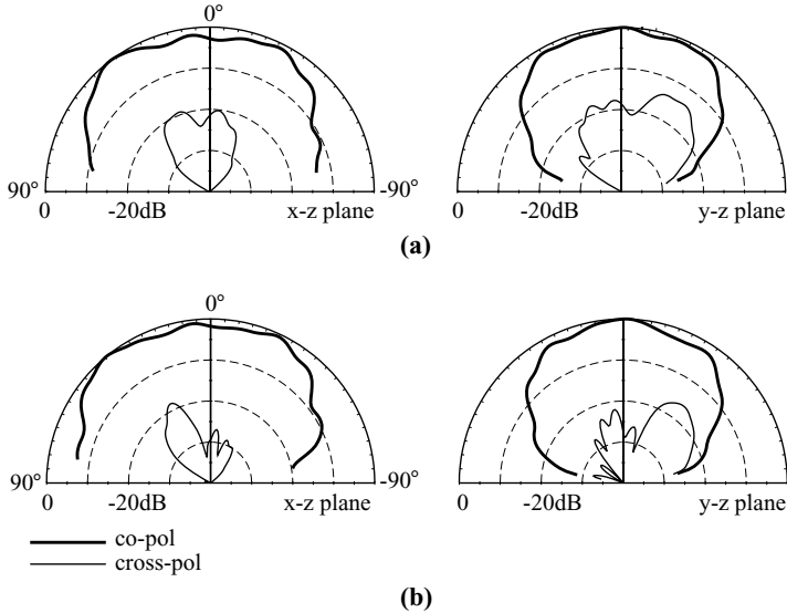
FIGURE 7.34 Measured E -plane ( x - z plane) and H -plane ( y - z plane) radiation patterns for the antenna studied in Figure 7.33. (a) f = 1742 MHz, (b) f = 1798 MHz. (From Ref. 21, © 1998 IEE, reprinted with permission.)
