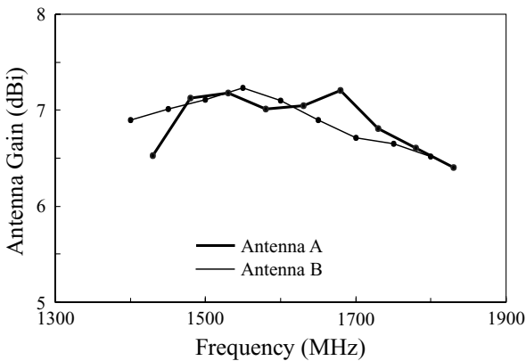
FIGURE 7.17 Measured antenna gain in the broadside direction for antennas A and B studied in Figure 7.15. (From Ref. 15, © 2001 IEEE, reprinted with permission.)
