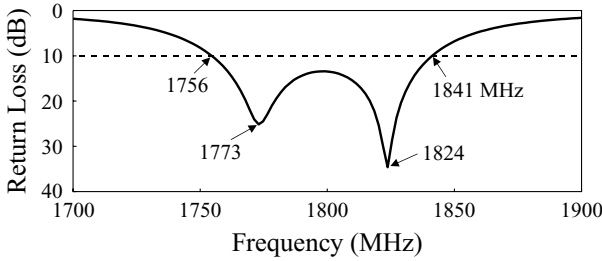
FIGURE 7.35 Measured return loss for the antenna shown in Figure 7.32; \epsilon_r = 4.4 , h = 1.6 mm, \ell_3 = 9 mm, \ell_4 = 8.5 mm, \ell_5 = 8 mm, and ground-plane size = 60 \times 50 mm 2 ; other parameters are given in Figure 7.32. (From Ref. [21], © 1998 IEE, reprinted with permission.)
