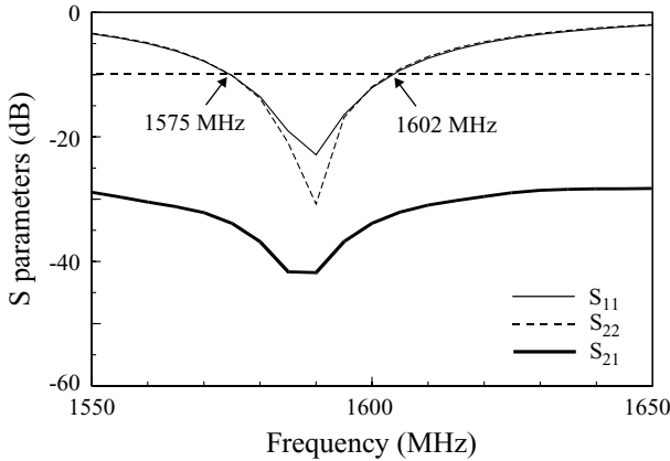
FIGURE 4.82 Measured S parameters for the antenna shown in Figure 4.81; \epsilon_r = 4.4 , h = 1.6 mm, L = 60 mm, (x_1, y_1) = (0, 8.7 mm), (x_2, y_2) = (-20.0, 1.5 mm), and ground-plane size = 75 \times 75 mm 2 .
