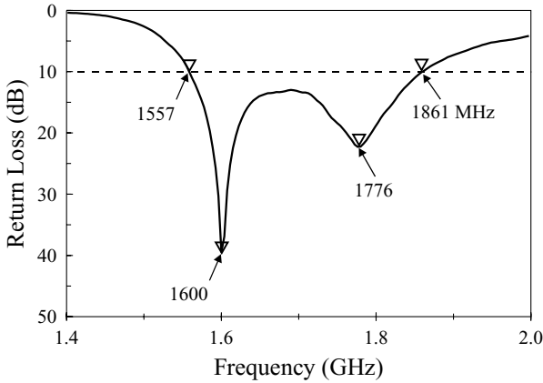
FIGURE 7.13 Measured return loss for the antenna shown in Figure 7.10; h = 14.3 mm, S = 3.2 mm, L_1 = 88.7 , L_2 = 80.4 mm, \alpha = 53.9^\circ , d_p = 26.2 mm, \ell_1 = 46.2 mm, \ell_2 = 20 mm, w_1 = 3.7 mm, and w_2 = 2.5 mm. (From Ref. 14, © 1997 IEEE, reprinted with permission.)
