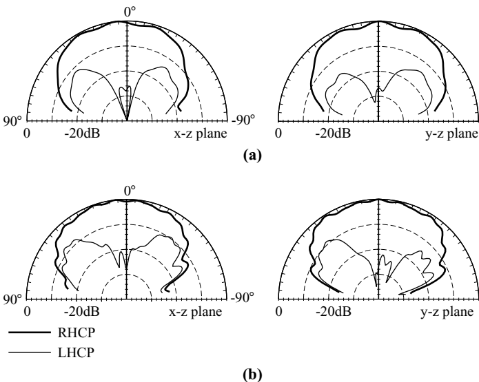
FIGURE 9.35 Measured radiation patterns for antenna B studied in Figure 9.32. (a) f_1 = 1632 \text{ MHz} , (b) f_2 = 2882 \text{ MHz} . (From Ref. 11, © 2001 IEEE, reprinted with permission.)
