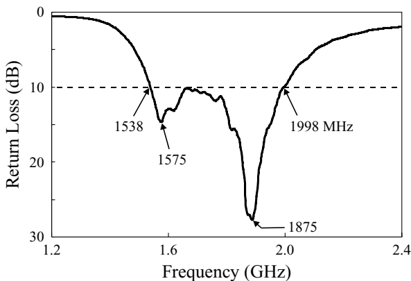
FIGURE 7.20 Measured return loss for the antenna shown in Figure 7.19; h = 12 mm, t = 0.8 mm, D = 76 mm, L = 47.8 mm, w = 5 mm, d_p = 16.8 mm, and ground-plane size = 150 \times 150 mm 2 . (From Ref. 17, © 2000 John Wiley & Sons, Inc.)
