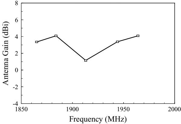
FIGURE 7.56 Measured antenna gain in the broadside direction for the antenna studied in Figure 7.54 with \phi_c = 40^\circ . (From Ref. 27, © 1999 John Wiley & Sons, Inc.)
