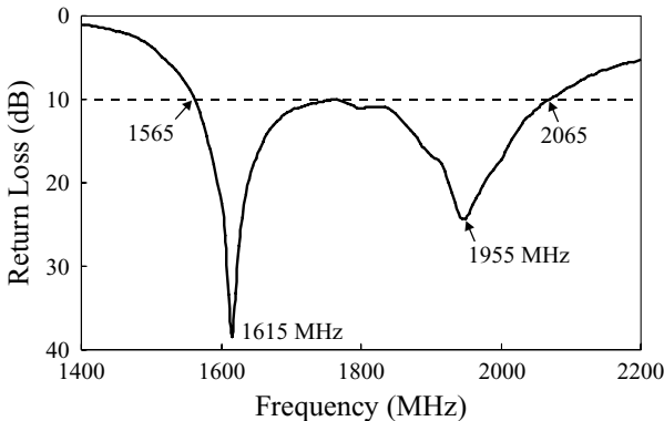
FIGURE 7.7 Measured return loss for the antenna shown in Figure 7.6.
