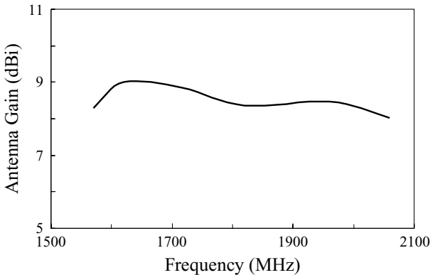
FIGURE 7.9 Measured antenna gain for the antenna shown in Figure 7.6.
