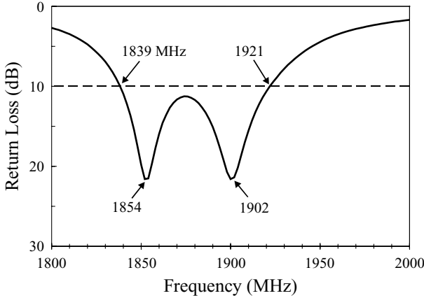
FIGURE 7.62 Measured return loss for the antenna shown in Figure 7.61; \epsilon_r = 4.4 , h = 1.6 mm, L = 50 mm, d_p = 22.3 mm, \ell_m = 3.5 mm, \ell_1 = 9.2 mm, w_1 = 7.3 mm, \ell_2 = 14.1 mm, and w_2 = 9.3 mm.
