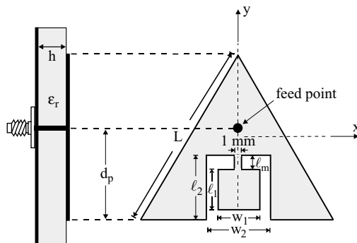
FIGURE 7.61 Geometry of a broadband equilateral-triangular microstrip antenna with integrated reactive loading.
