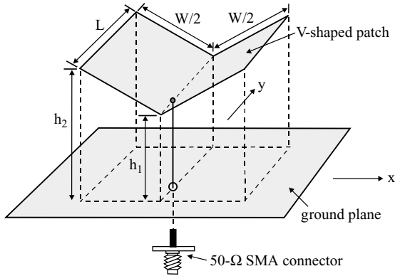
FIGURE 7.28 Geometry of a broadband probe-fed microstrip antenna with a V-shaped patch.
