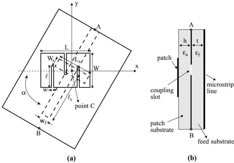
FIGURE 4.66 (a) Top view and (b) cross-sectional view of a slot-coupled, meandered rectangular microstrip antenna for compact dual-frequency operation. (From Ref. 33, © 1998 IEE, reprinted with permission.)
