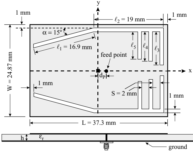
FIGURE 7.32 Geometry of a broadband rectangular microstrip antenna with a pair of toothbrush-shaped slots. (From Ref. 21, © 1998 IEE, reprinted with permission.)
