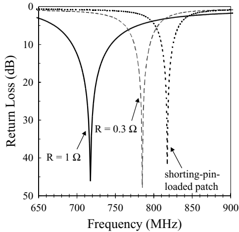
FIGURE 3.32 Measured return loss for the antenna shown in Figure 3.31 with chip-resistor loading only; antenna parameters are given in Table 3.4. (From Ref. 18, © 1998 John Wiley & Sons, Inc.)
