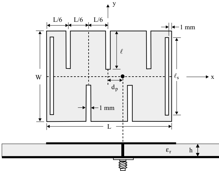
FIGURE 4.29 Geometry of a slot-loaded, meandered rectangular microstrip antenna with compact dual-frequency operation. (From Ref. 17, © 1998 IEE, reprinted with permission.)
