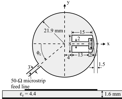
FIGURE 7.53 Geometry of a microstrip-line-fed broadband circular microstrip antenna with embedded reactive loading. The dimensions (in millimeters) in the figure are not to scale. (From Ref. 27, © 1999 John Wiley & Sons, Inc.)
