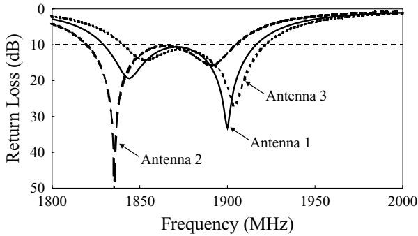
FIGURE 7.40 Measured return loss for the antenna shown in Figure 7.39 with an FR4 substrate. Parameters for antennas 1–3 are given in Table 7.1. (From Ref. 23, © 2000 IEEE, reprinted with permission.)
