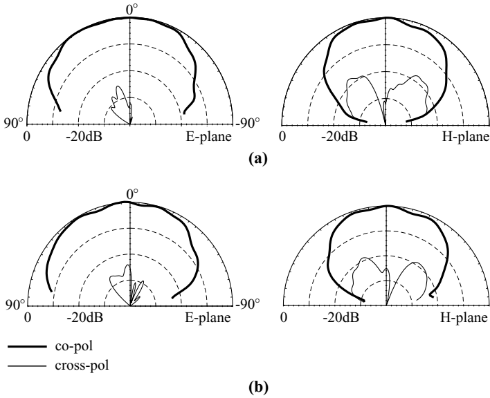
FIGURE 2.12 Measured E -plane ( x - z plane) and H -plane ( y - z plane) radiation patterns for the compact microstrip antenna studied in Figure 2.11. (a) Antenna 3 ( \ell_1 = 12 mm) at 1723 MHz, (b) antenna 4 ( \ell_1 = 14 mm) at 1587 MHz. (From Ref. 9, © 2001 John Wiley & Sons, Inc.)
