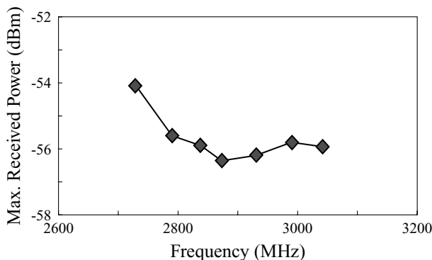
FIGURE 7.4 Measured maximum received power in the broadside direction for the antenna studied in Figure 7.2. (From Ref. 3, © 1999 John Wiley & Sons, Inc.)
