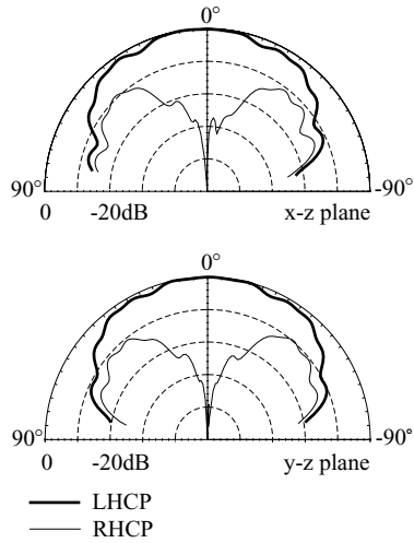
FIGURE 5.62 Measured radiation patterns for the antenna studied in Figure 5.61 with f = 2504 MHz. (From Ref. 19, © 1998 IEE, reprinted with permission.)
