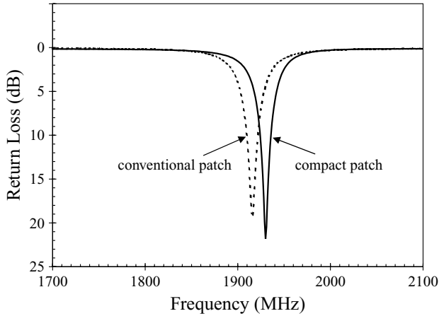
FIGURE 2.3 Measured return loss of shorted and conventional triangular microstrip antennas. The solid line is for a shorted antenna with d = 15.3 mm, and d_s = 13.25 mm, and d_p = 12.75 mm; the dashed line is for a conventional antenna with d = 59.9 mm and d_p = 24.1 mm. (From Ref. 7, © 1997 IEE, reprinted with permission.)
