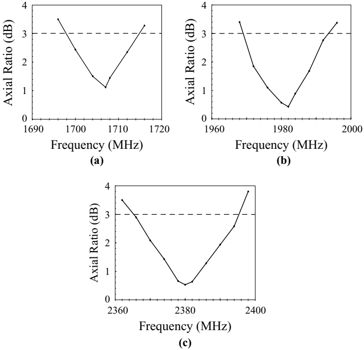
FIGURE 5.47 Measured axial ratio for the antennas studied in Figure 5.46. (From Ref. 14, © 1998 IEE, reprinted with permission.)
