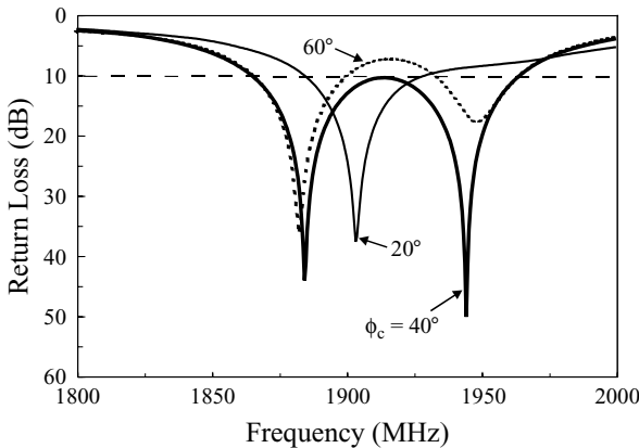
FIGURE 7.54 Measured return loss for the antenna shown in Figure 7.53 with various angles \phi_c ; \epsilon_r = 4.4 , h = 1.6 \text{ mm} , d = 21.9 \text{ mm} , and ground-plane size = 75 \times 75 \text{ mm}^2 . (From Ref. 27, © 1999 John Wiley & Sons, Inc.)
