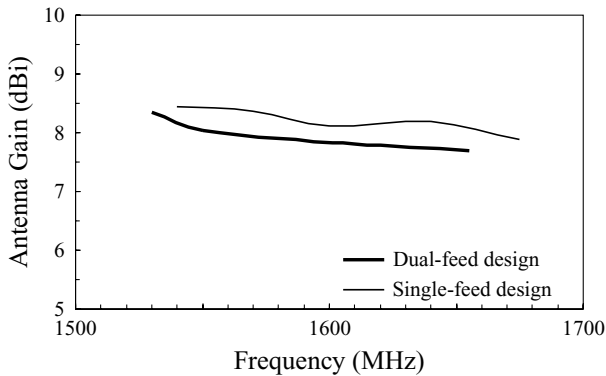
FIGURE 7.67 Measured on-axis antenna gain for the antenna studied in Figure 7.65. (From Ref. 10, © 2000 John Wiley & Sons, Inc.)
