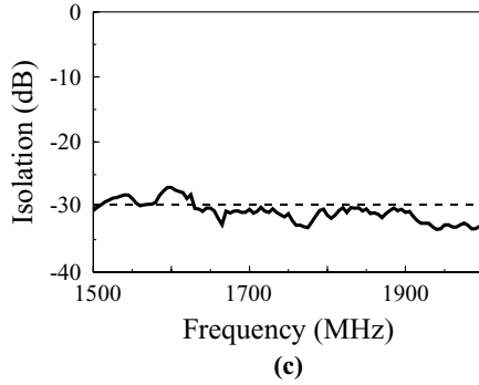
FIGURE 8.15 (Continued.) (c) isolation between ports 1 and 2.
