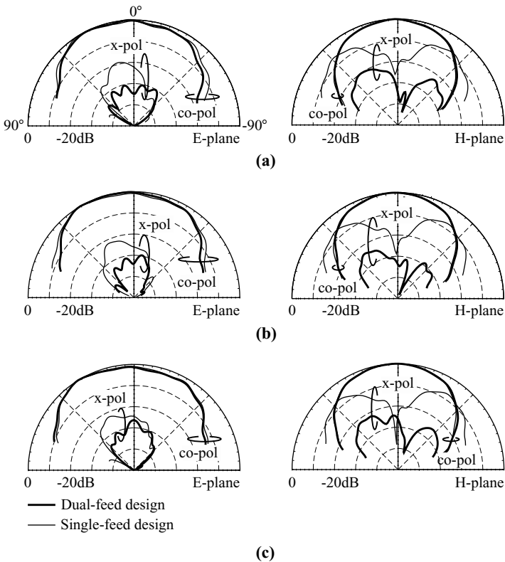
FIGURE 7.69 Measured E -plane ( x - z plane) and H -plane ( y - z plane) radiation patterns for the antenna studied in Figure 7.68. (a) f = 1748 MHz, (b) f = 1800 MHz, (c) f = 1880 MHz. (From Ref. 10, © 2000 John Wiley & Sons, Inc.)
