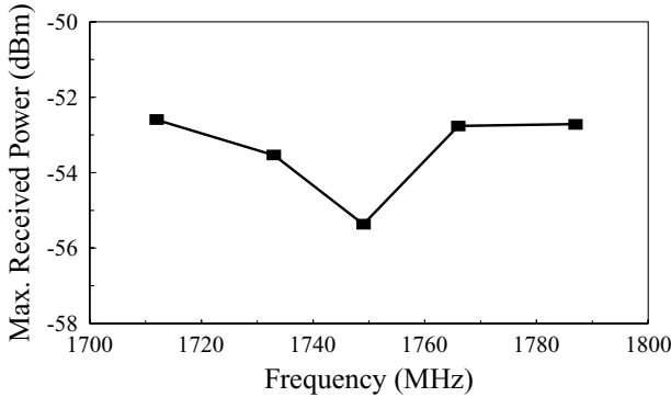
FIGURE 7.60 Measured maximum received power in the broadside direction for the antenna shown in Figure 7.57 with \alpha = 30^\circ . (From Ref. 28, © 1999 John Wiley & Sons, Inc.)
