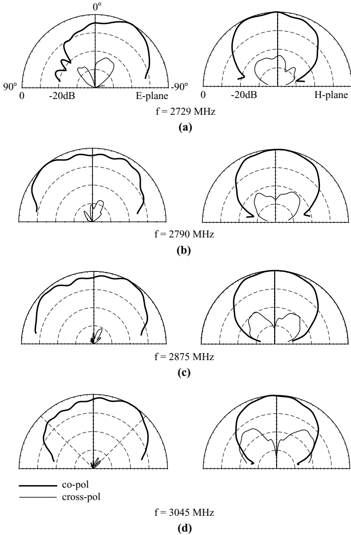
FIGURE 7.3 Measured E -plane ( y - z plane) and H -plane ( x - z plane) radiation patterns for the antenna studied in Figure 7.2. (a) f = 2729 \text{ MHz} , (b) f = 2790 \text{ MHz} , (c) f = 2875 \text{ MHz} , (d) f = 3045 \text{ MHz} . (From Ref. 3, © 1999 John Wiley & Sons, Inc.)
