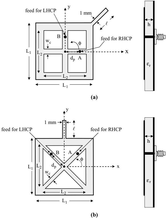
FIGURE 5.66 Geometries of square-ring microstrip antennas with a cross strip for compact CP operation. (a) The case with a centerline cross strip, (b) the case with a diagonal cross strip. (From Ref. 20, © 1999 IEEE, reprinted with permission.)
