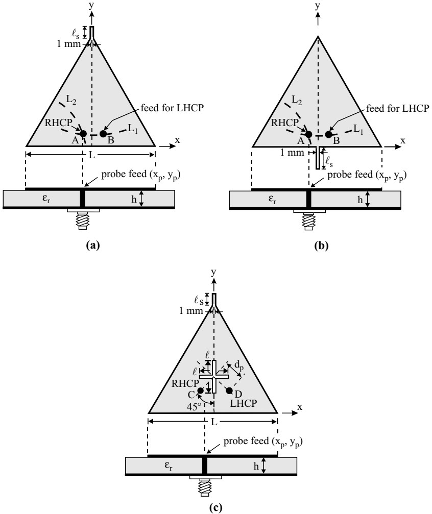
FIGURE 5.69 Geometries of single-feed circularly polarized equilateral-triangular microstrip antennas. (a) With a tuning stub at the triangle tip, (b) with a tuning stub at the bottom edge of the triangular patch, and (c) with a tuning stub at the triangle tip and a cross slot at the patch center. (From Ref. 21, © 2000 IEEE, reprinted with permission.)
