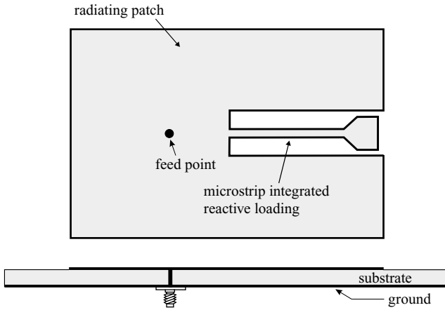
FIGURE 7.48 Geometry of a broadband rectangular microstrip antenna with an inserted integrated reactive loading.
