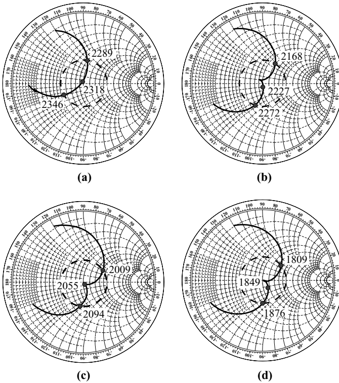
FIGURE 5.31 Measured input impedance for the antenna with slits of different lengths; \epsilon_r = 4.4 , h = 1.6 mm, L = 30 mm, and feed at point C. (a) l_x = l_y = 0 ; (b) l_x = 10 mm, l_y = 6.4 mm; (c) l_x = 15 mm, l_y = 13.1 mm; (d) l_x = 20 mm, l_y = 18.4 mm. (From Ref. 8, © 1997 IEE, reprinted with permission.)
