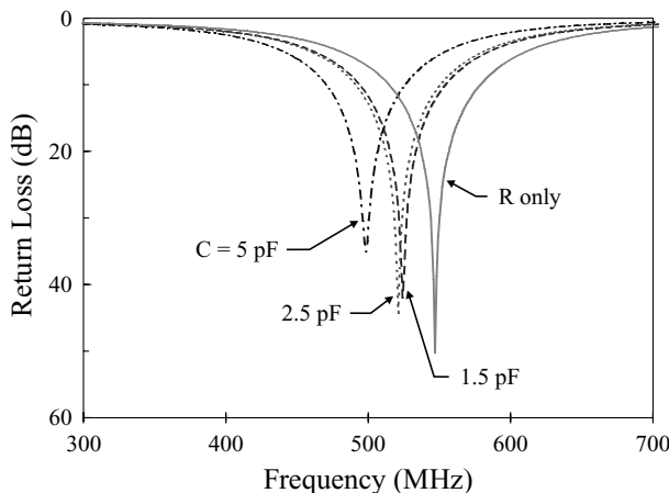
FIGURE 3.28 Measured return loss for the antenna shown in Figure 3.25 with chip-resistor and chip-capacitor loading; \epsilon_r = 4.4 , h = 1.6 mm, d = 21.97 mm, R = 1 \Omega , (x_R, y_R) = (0, 21 mm), (x_C, y_C) = (0, -21 mm), (x_p, y_p) = (0, -11.5 mm), and \phi_s = 180^\circ .
