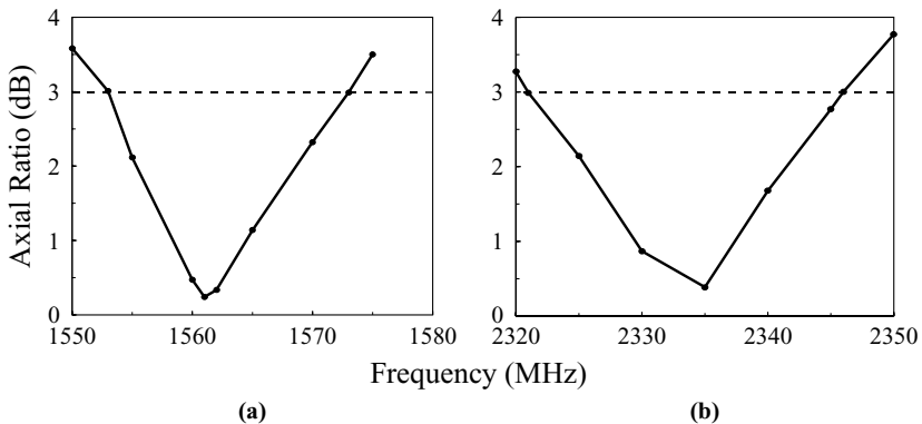
FIGURE 9.24 Measured axial ratio for the antenna studied in Figure 9.23. (a) The lower band; (b) the upper band. (From Ref. 10, © 1998 IEE, reprinted with permission.)
