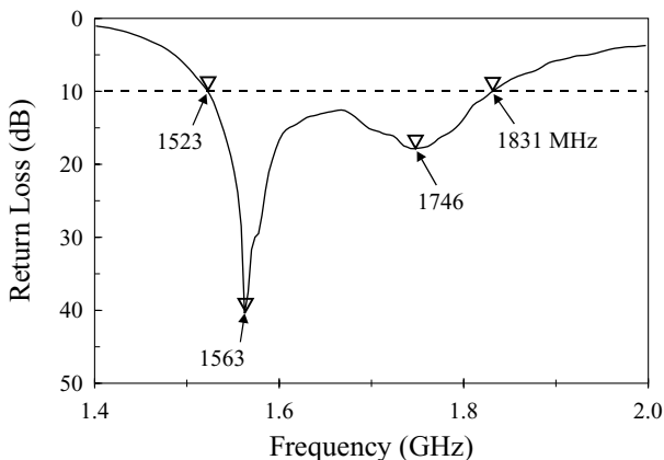
FIGURE 7.11 Measured return loss for the antenna shown in Figure 7.10; h = 14.3 mm, S = 3.2 mm, L_1 = L_2 = 91 mm, \alpha = 60^\circ , d_p = 26.2 mm, \ell_1 = 46.2 mm, \ell_2 = 24 mm, w_1 = 6 mm, and w_2 = 2.5 mm. (From Ref. 14, © 1997 IEE, reprinted with permission.)
