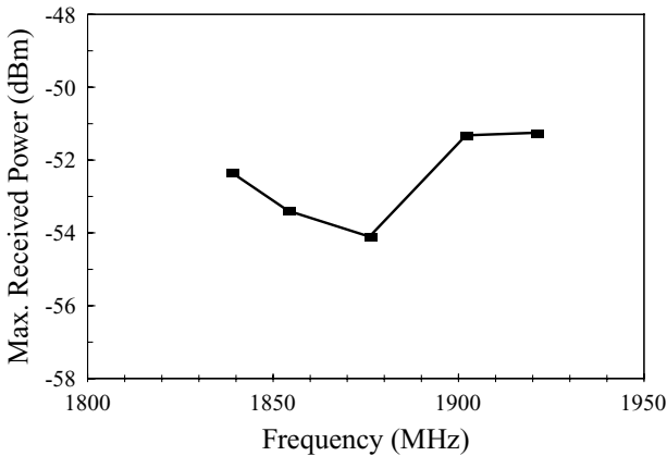
FIGURE 7.63 Measured on-axis maximum received power for the antenna studied in Figure 7.62.
