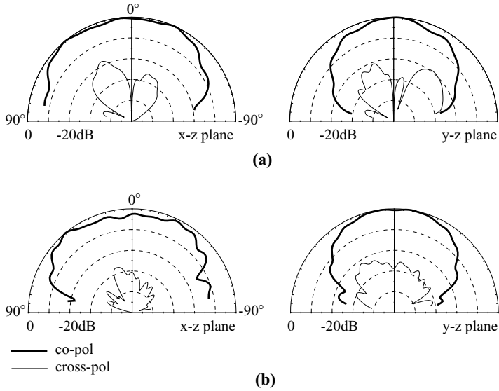
FIGURE 4.4 Measured E -plane ( x - z plane) and H -plane ( y - z plane) radiation patterns for the antenna studied in Figure 4.2 with \alpha = 15^\circ . (a) f = 1780 MHz, (b) f = 2304 MHz. (From Ref. 8, © 1998 IEE, reprinted with permission.)
