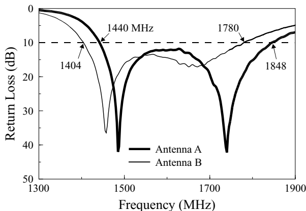
FIGURE 7.15 Measured return loss for the antenna shown in Figure 7.14; L = 65 mm, W = 105 mm, and ground-plane size = 150 \times 150 mm 2 . Antenna A: h = 14.3 mm, \ell = 47 mm, w_1 = 6.3 mm, w_2 = 15.3 mm, and d_p = 10 mm. Antenna B: h = 15.7 mm, \ell = 53 mm, w_1 = 10 mm, w_2 = 8 mm, and d_p = 13 mm. (From Ref. 15, © 2001 IEEE, reprinted with permission.)
