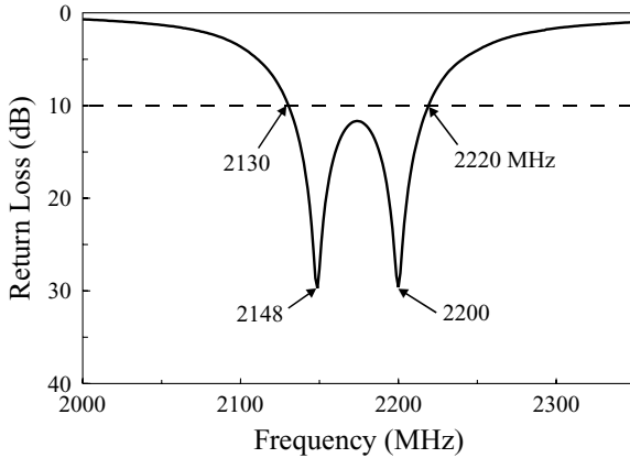
FIGURE 7.45 Measured return loss for the antenna shown in Figure 7.44; \epsilon_r = 4.4 , h = 1.6 mm, d_p = 13 mm, \phi = 32^\circ , and ground-plane size = 75 \times 75 mm 2 . Other parameters are given in Figure 7.44. (From Ref. 24, © 1999 John Wiley & Sons, Inc.)
