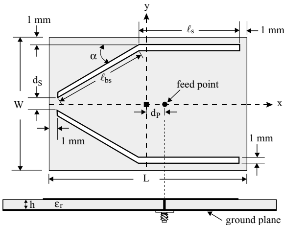
FIGURE 4.1 Geometry of a dual-frequency rectangular microstrip antenna with a pair of bent slots placed close to the patch's nonradiating edges. (From Ref. 8, © 1998 IEE, reprinted with permission.)
