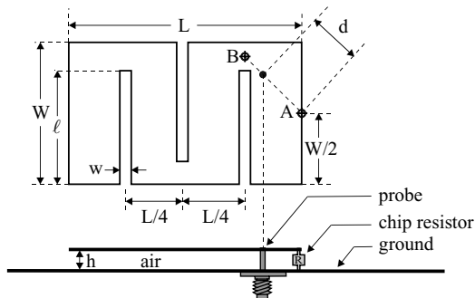
FIGURE 3.41 Geometry of a meandered PIFA with a chip resistor. (From Ref. 21, © 1998 IEE, reprinted with permission.)
