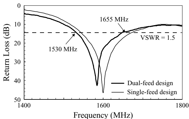
FIGURE 7.65 Measured return loss for the antenna shown in Figure 7.64; h = 15 mm, L = 60 mm, W = 90 mm, \ell = 13.5 mm, g = 1.8 mm, d = 16.8 mm, w_c = 1.0 mm, and ground-plane size = 150 \times 150 mm 2 . (From Ref. 10, © 2000 John Wiley & Sons, Inc.)
