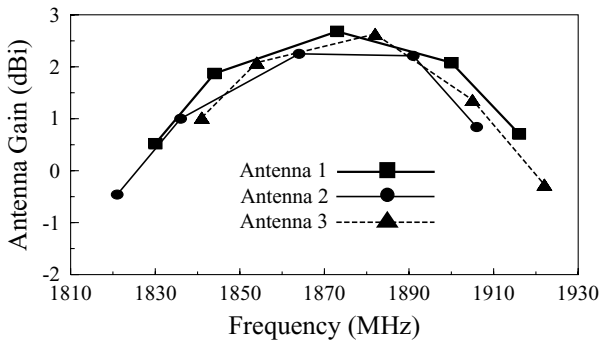
FIGURE 7.42 Measured peak antenna gain for antennas 1–3 studied in Figure 7.40. (From Ref. 23, © 2000 IEEE, reprinted with permission.)
