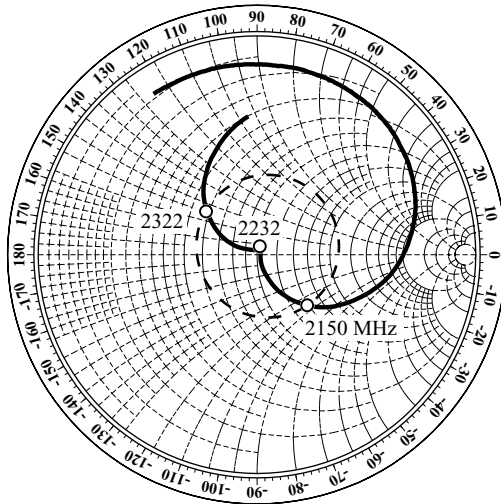
FIGURE 9.2 Measured input impedance on a Smith chart for the antenna shown in Figure 9.1; \epsilon_1 = \epsilon_2 = 4.4 , h_1 = 0.8 mm, h_2 = 1.6 mm, w_f = 1.5 mm, t = 23 mm, S = 5 mm, S_{arm} = 6.2 mm, L = 33.5 mm, and W = 30 mm. (From Ref. 1, © 1998 IEE, reprinted with permission.)
