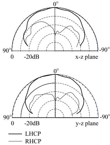
FIGURE 5.65 Measured radiation patterns for the antenna studied in Figure 5.64 with f = 1587 MHz. (From Ref. 19, © 1998 IEE, reprinted with permission.)
