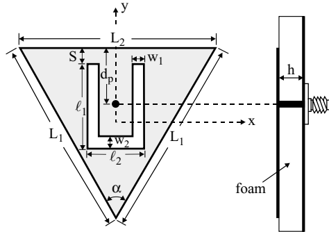
FIGURE 7.10 Geometry of a broadband probe-fed triangular microstrip antenna with a U-shaped slot. (From Ref. 14, © 1997 IEE, reprinted with permission.)
