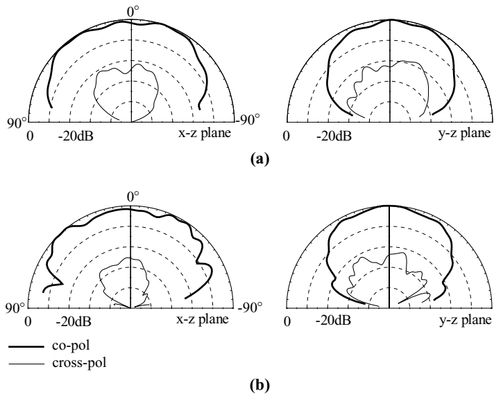
FIGURE 4.5 Measured E -plane ( x - z plane) and H -plane ( y - z plane) radiation patterns for the antenna studied in Figure 4.2 with \alpha = 30^\circ . (a) f = 1528 MHz, (b) f = 2448 MHz. (From Ref. 8, © 1998 IEE, reprinted with permission.)
